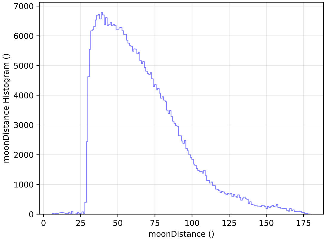
too_elab_heavy_r64_d3_gz_v3.4_10yrs WFD y band: moonDistance Histogram
