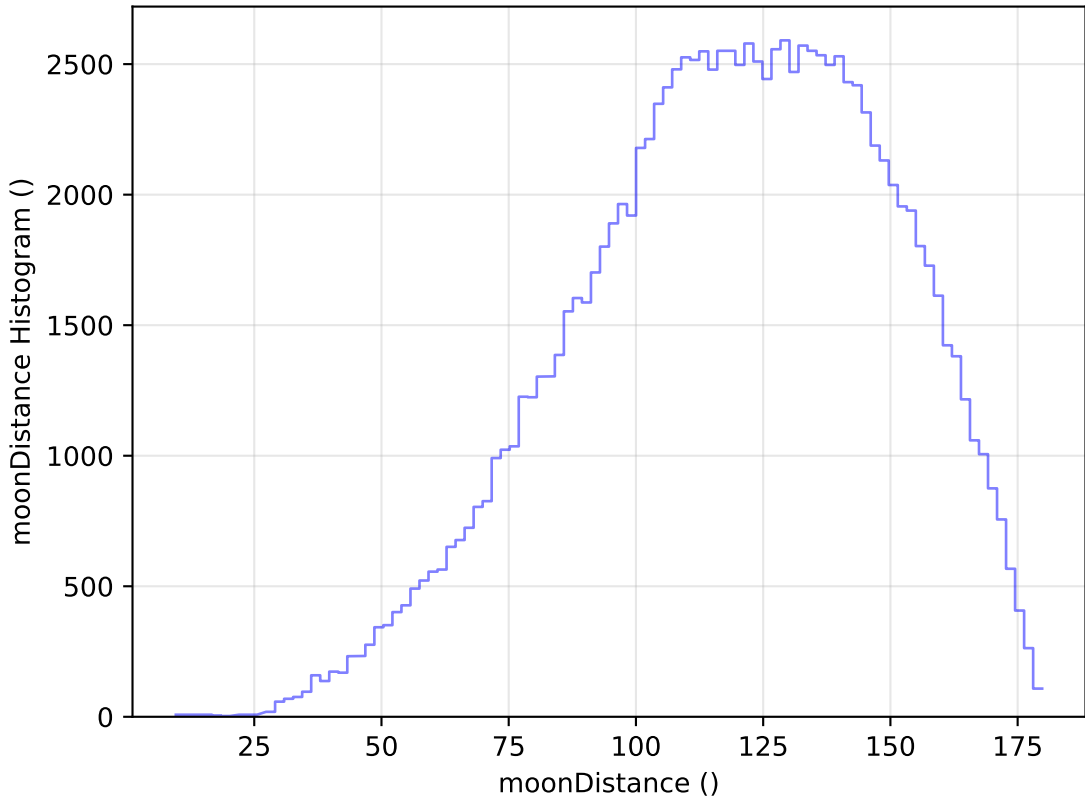
too_elab_heavy_r64_d3_gz_v3.4_10yrs WFD u band: moonDistance Histogram
