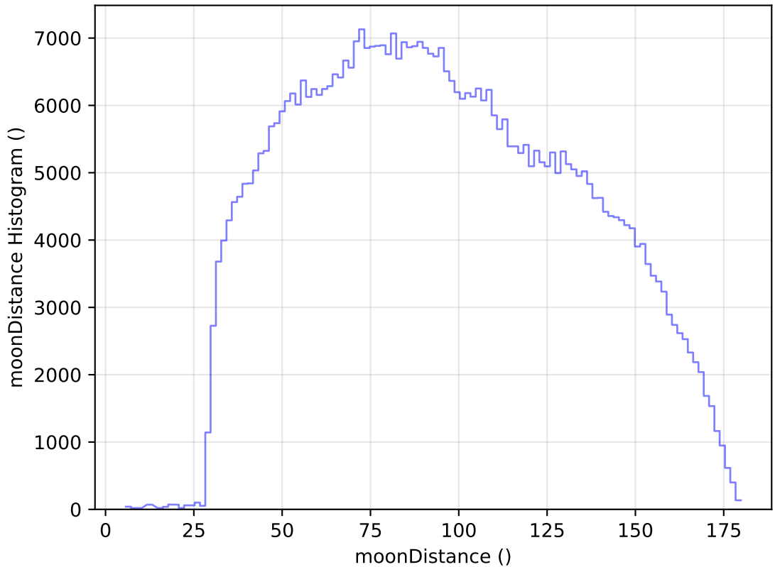
too_elab_heavy_r64_d3_gz_v3.4_10yrs WFD i band: moonDistance Histogram
