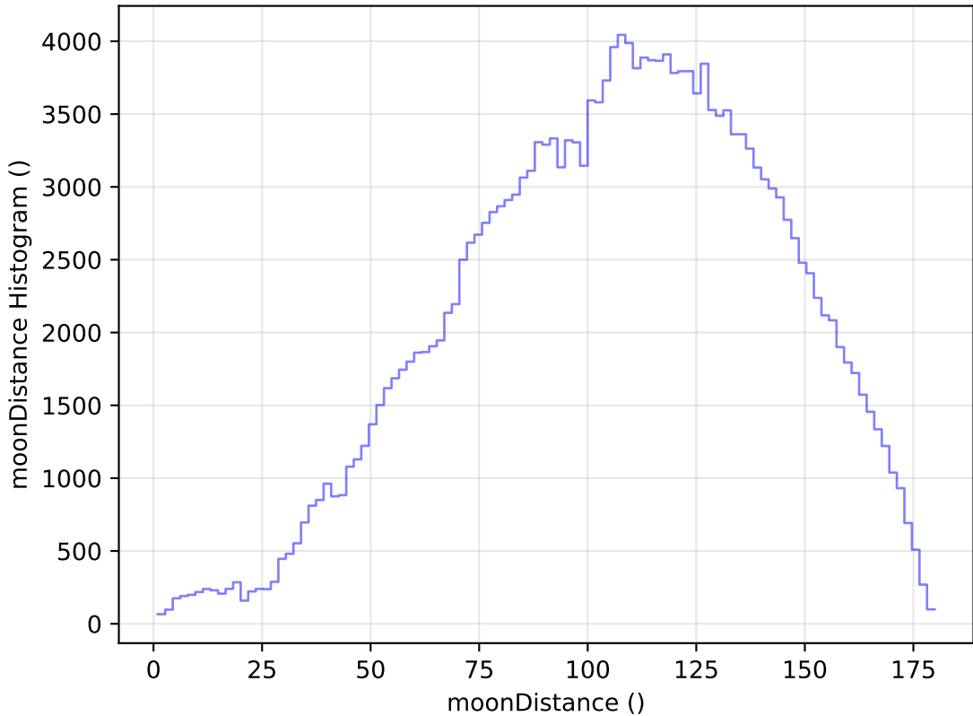
too_elab_heavy_r64_d3_gz_v3.4_10yrs WFD g band: moonDistance Histogram
