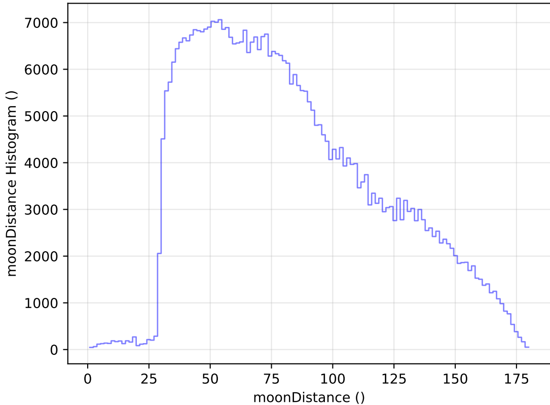
too_elab_heavy_r64_d3_gz_v3.4_10yrs All sky z band: moonDistance Histogram
