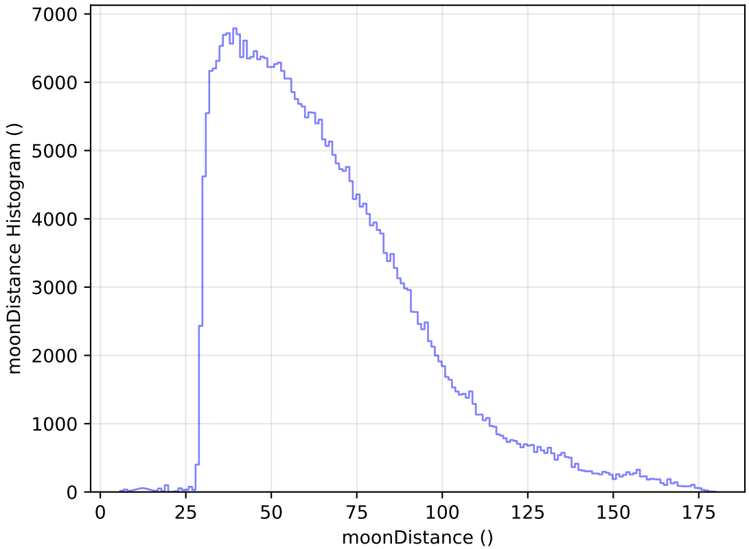
too_elab_heavy_r64_d3_gz_v3.4_10yrs All sky y band: moonDistance Histogram
