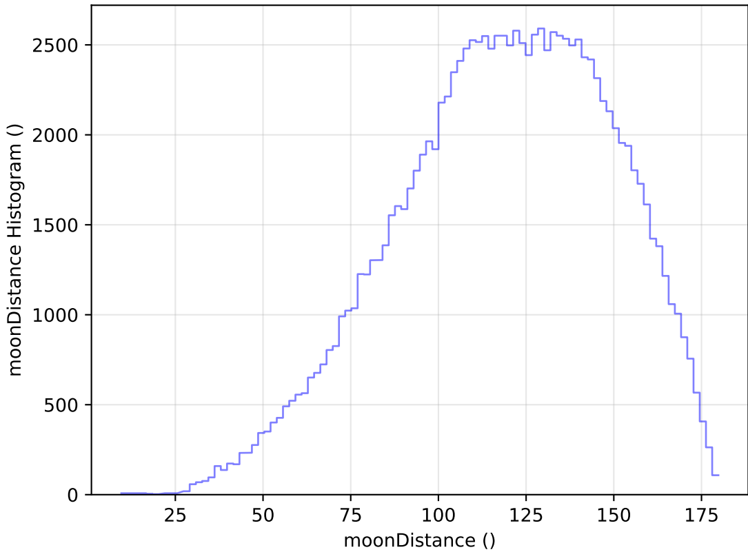
too_elab_heavy_r64_d3_gz_v3.4_10yrs All sky u band: moonDistance Histogram
