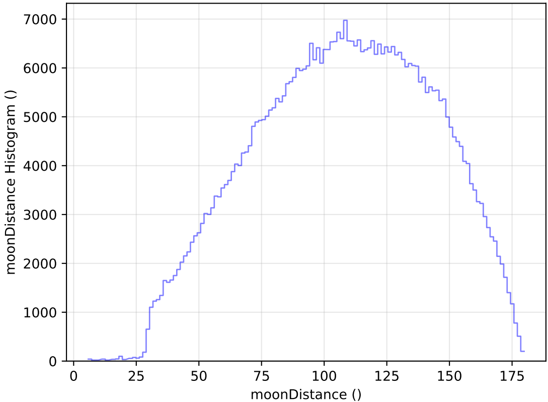
too_elab_heavy_r64_d3_gz_v3.4_10yrs All sky r band: moonDistance Histogram
