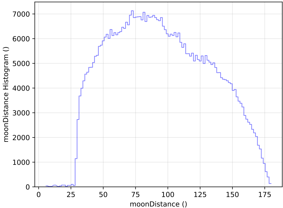
too_elab_heavy_r64_d3_gz_v3.4_10yrs All sky i band: moonDistance Histogram
