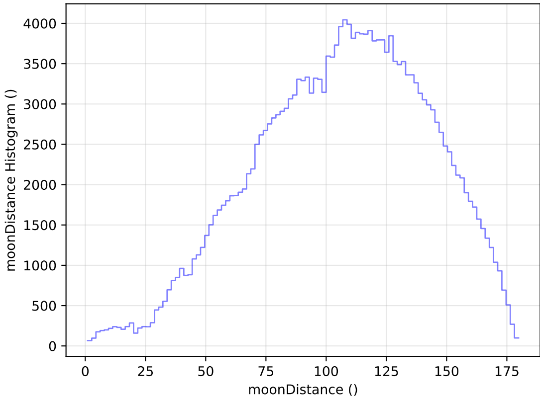
too_elab_heavy_r64_d3_gz_v3.4_10yrs All sky g band: moonDistance Histogram
