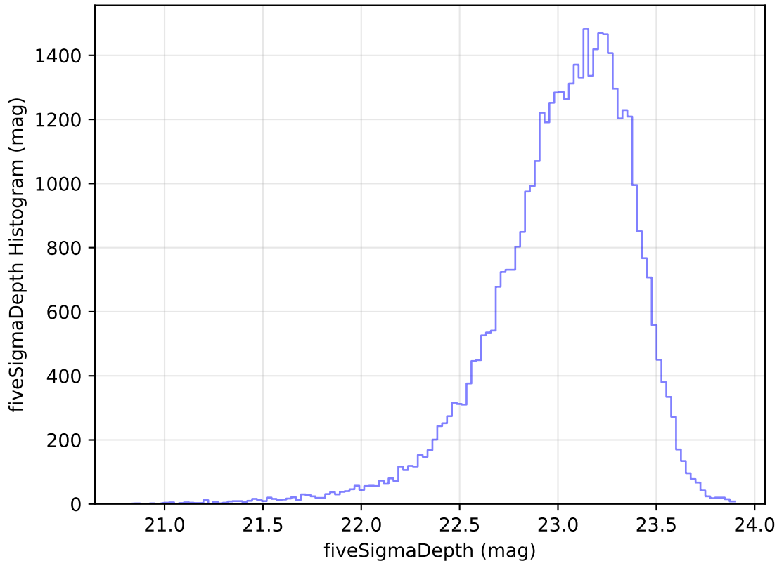
too_elab_heavy_r64_d3_gz_v3.4_10yrs Yr 1 z band: fiveSigmaDepth Histogram
