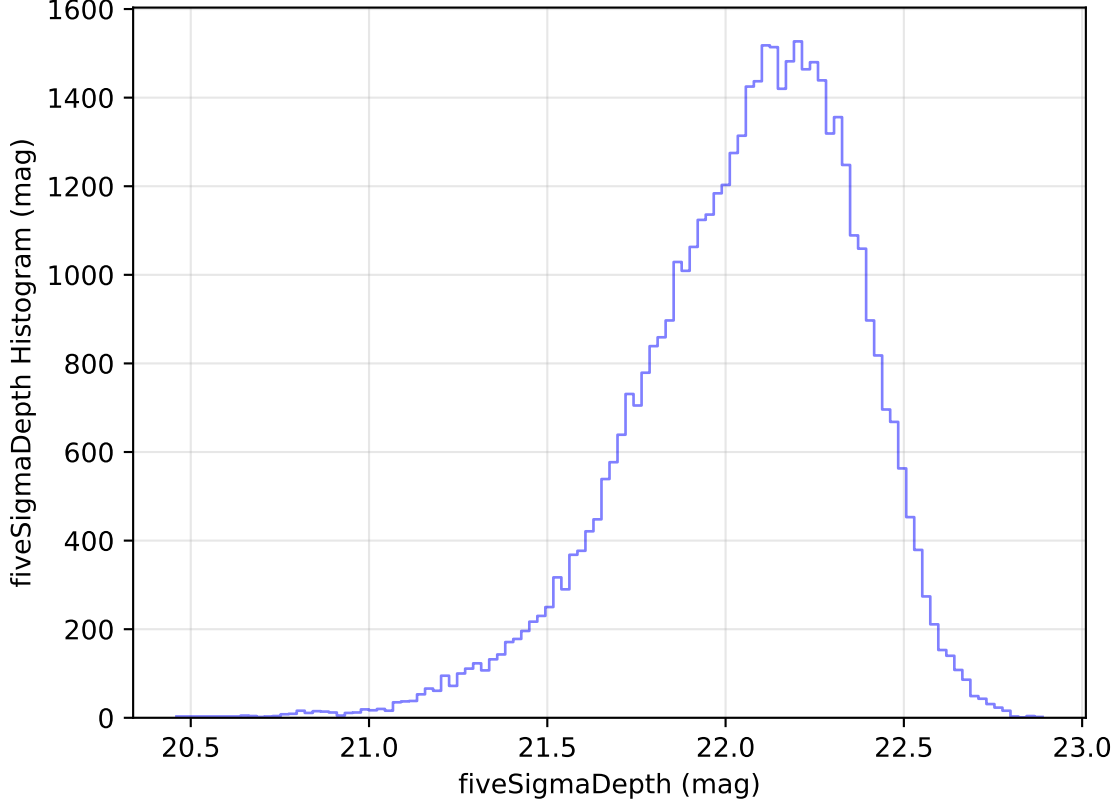
too_elab_heavy_r64_d3_gz_v3.4_10yrs Yr 1 y band: fiveSigmaDepth Histogram
