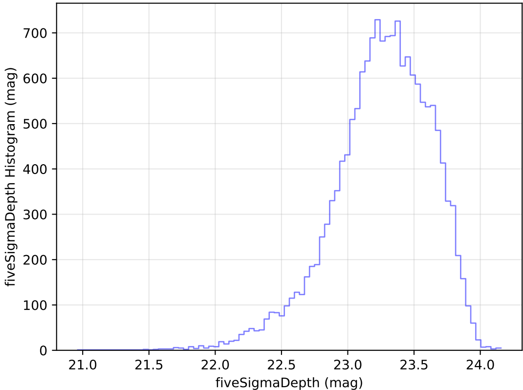
too_elab_heavy_r64_d3_gz_v3.4_10yrs Yr 1 u band: fiveSigmaDepth Histogram
