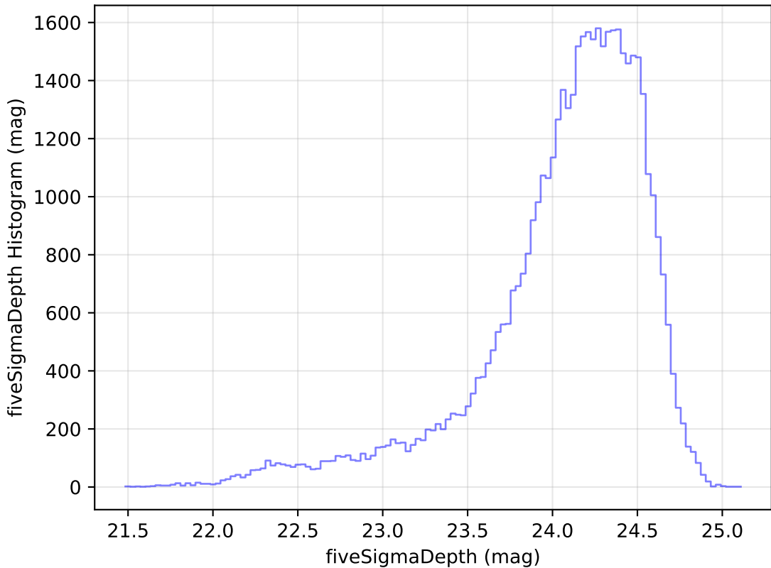
too_elab_heavy_r64_d3_gz_v3.4_10yrs Yr 1 r band: fiveSigmaDepth Histogram
