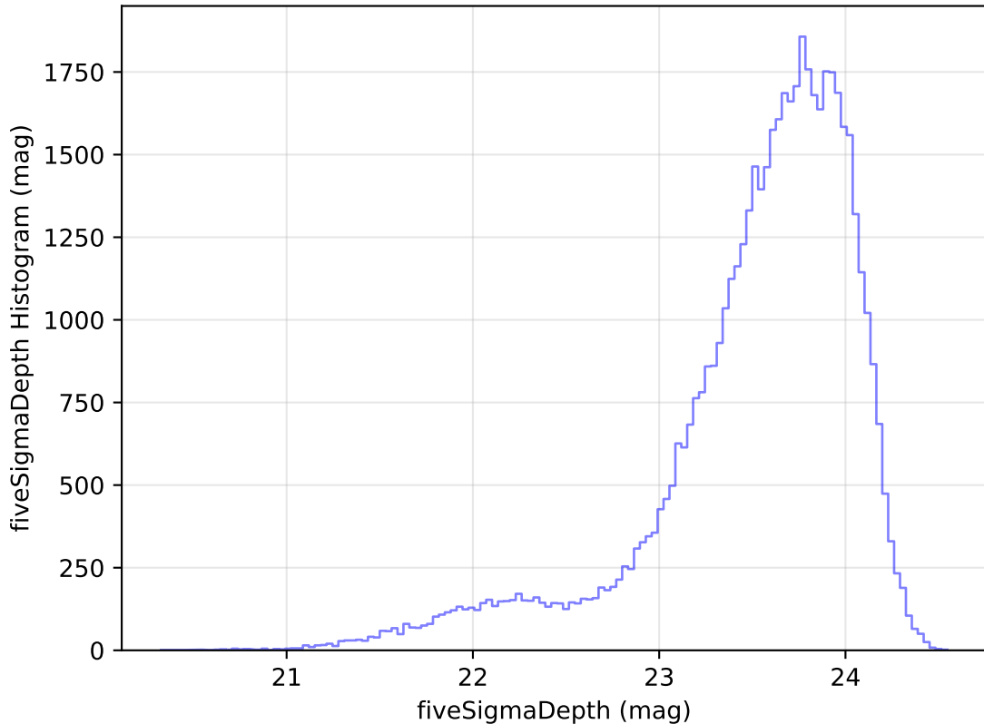
too_elab_heavy_r64_d3_gz_v3.4_10yrs Yr 1 i band: fiveSigmaDepth Histogram
