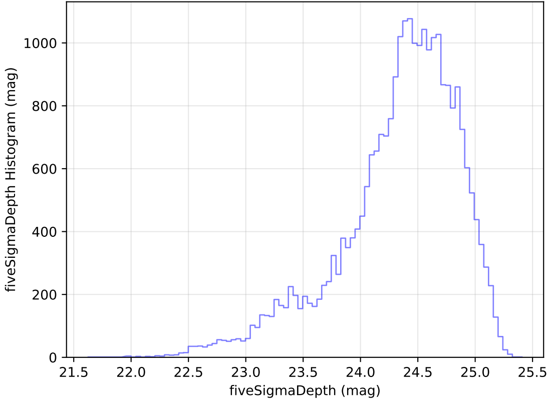
too_elab_heavy_r64_d3_gz_v3.4_10yrs Yr 1 g band: fiveSigmaDepth Histogram
