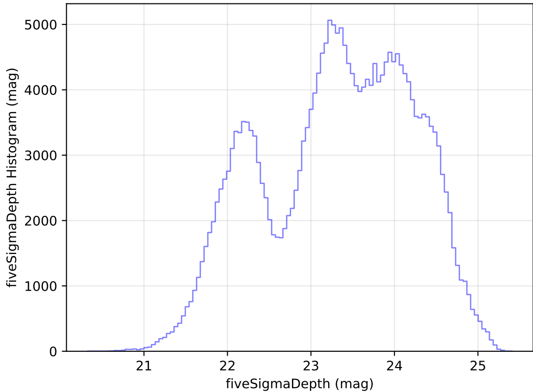
too_elab_heavy_r64_d3_gz_v3.4_10yrs Yr 1 all bands: fiveSigmaDepth Histogram
