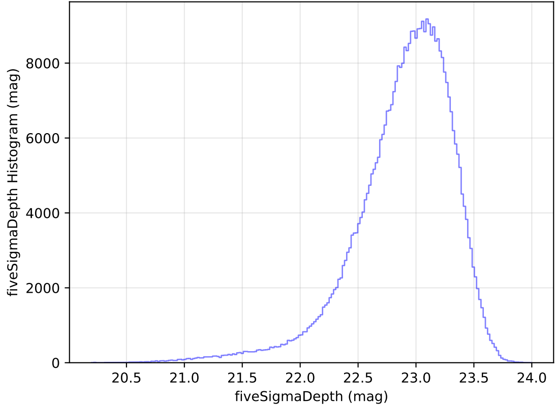
too_elab_heavy_r64_d3_gz_v3.4_10yrs WFD z band: fiveSigmaDepth Histogram
