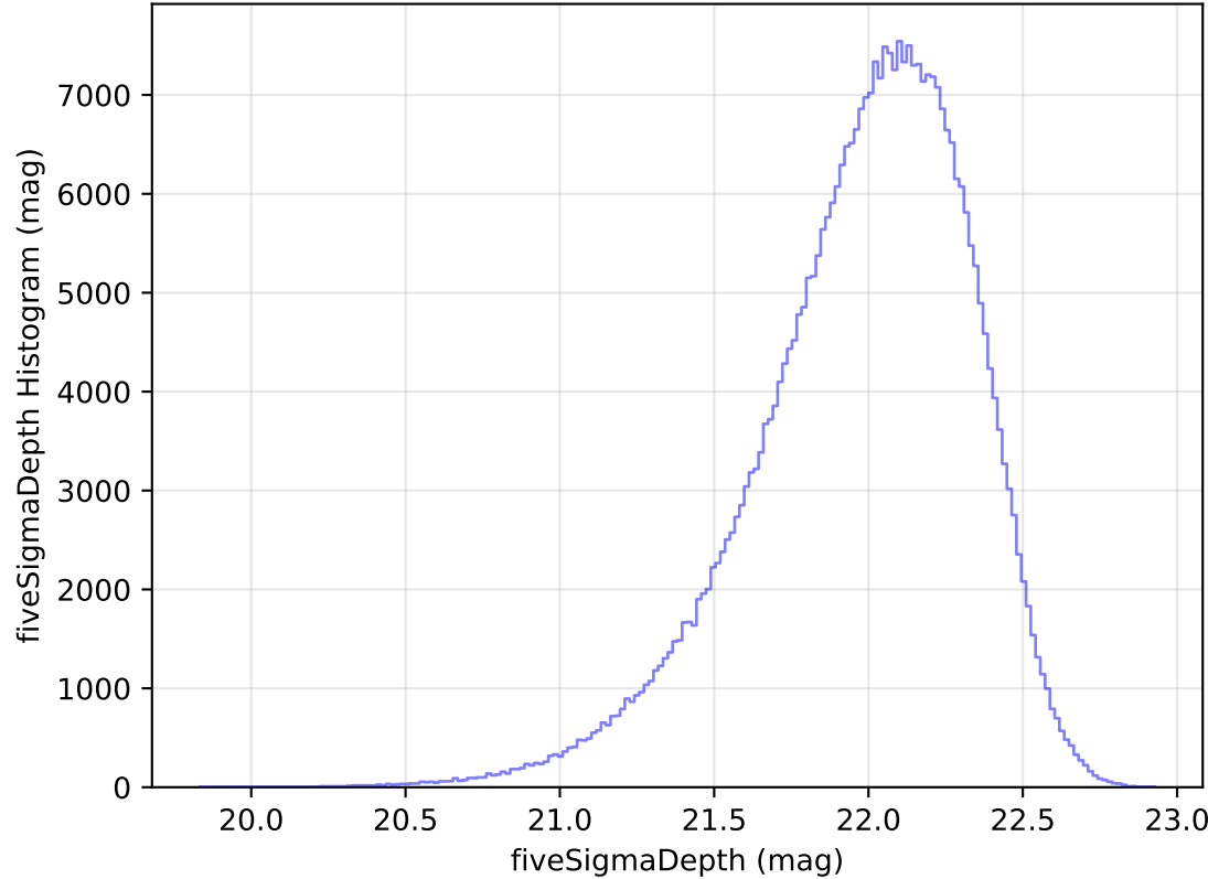
too_elab_heavy_r64_d3_gz_v3.4_10yrs WFD y band: fiveSigmaDepth Histogram
