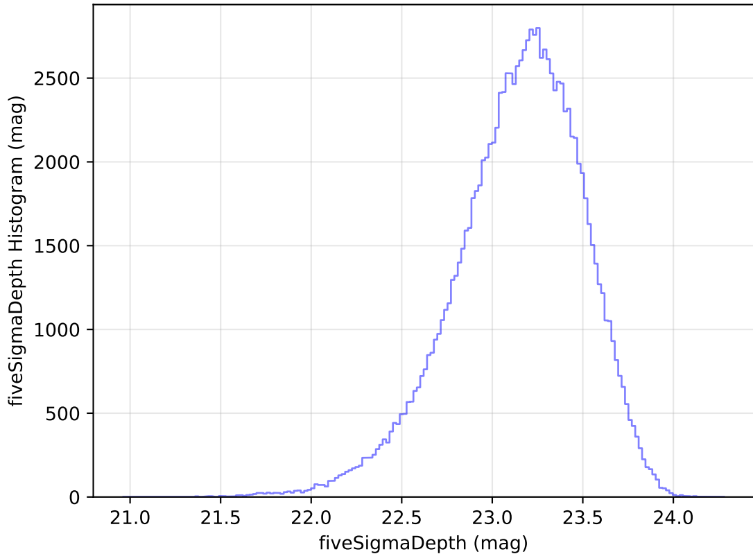
too_elab_heavy_r64_d3_gz_v3.4_10yrs WFD u band: fiveSigmaDepth Histogram
