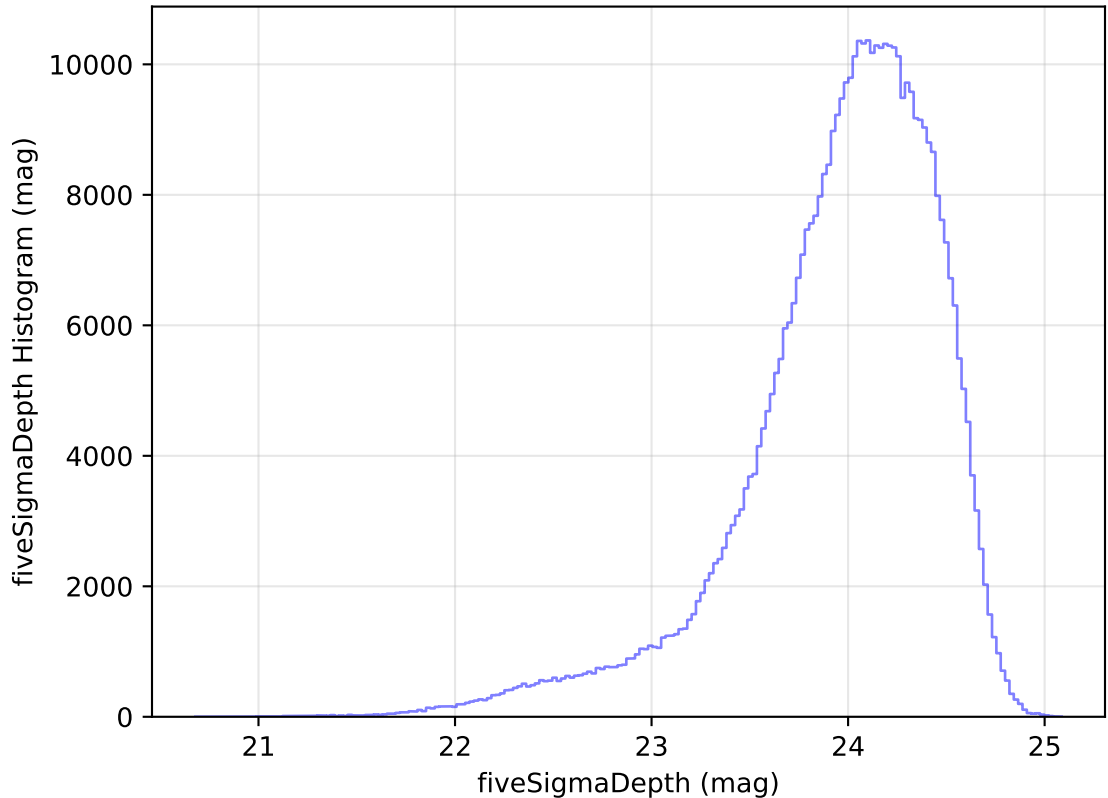
too_elab_heavy_r64_d3_gz_v3.4_10yrs WFD r band: fiveSigmaDepth Histogram
