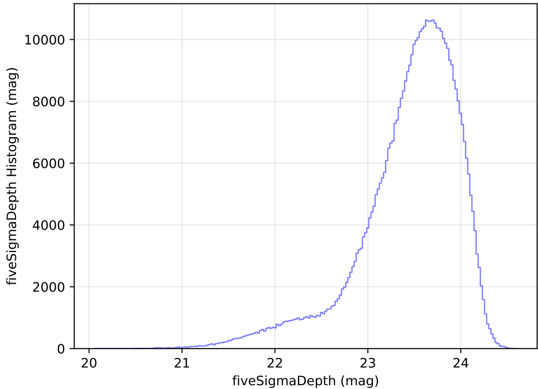
too_elab_heavy_r64_d3_gz_v3.4_10yrs WFD i band: fiveSigmaDepth Histogram
