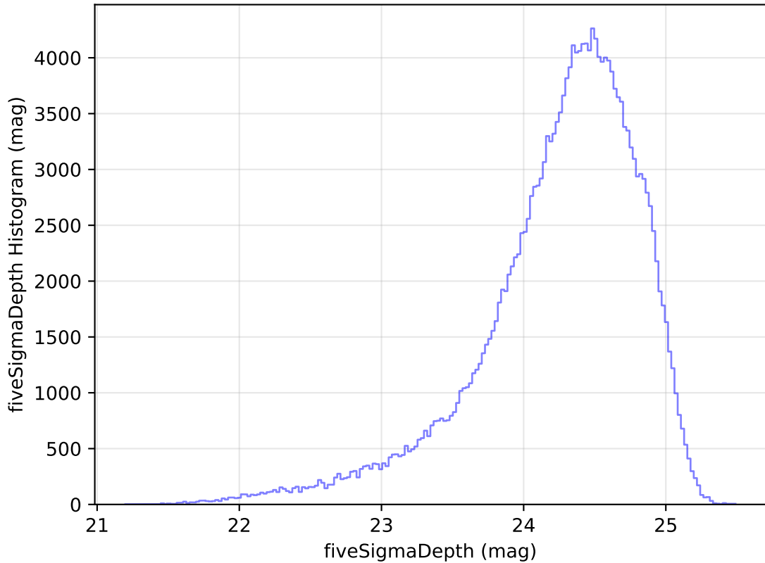
too_elab_heavy_r64_d3_gz_v3.4_10yrs WFD g band: fiveSigmaDepth Histogram
