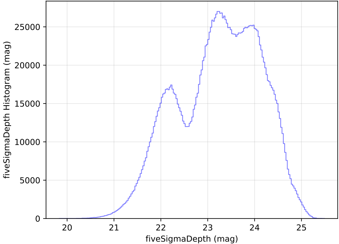
too_elab_heavy_r64_d3_gz_v3.4_10yrs WFD all bands: fiveSigmaDepth Histogram
