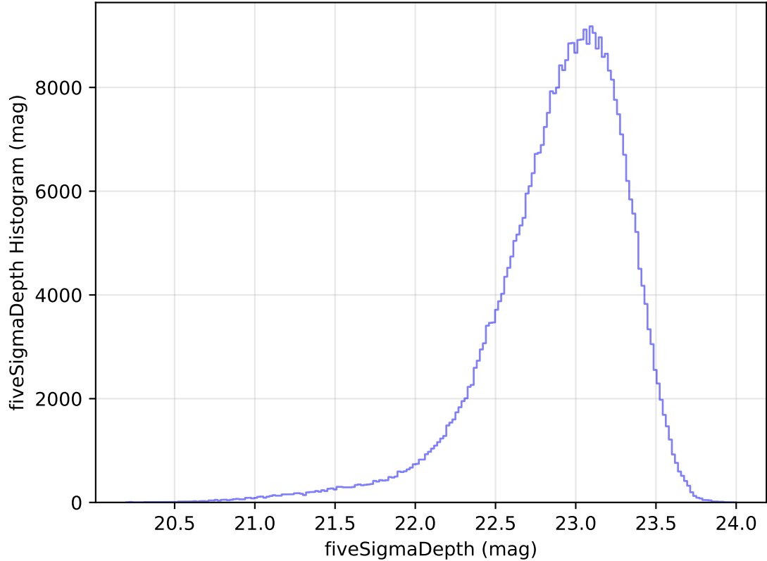
too_elab_heavy_r64_d3_gz_v3.4_10yrs All sky z band: fiveSigmaDepth Histogram
