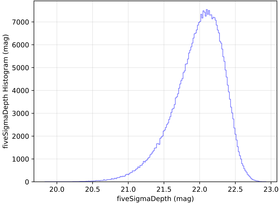
too_elab_heavy_r64_d3_gz_v3.4_10yrs All sky y band: fiveSigmaDepth Histogram
