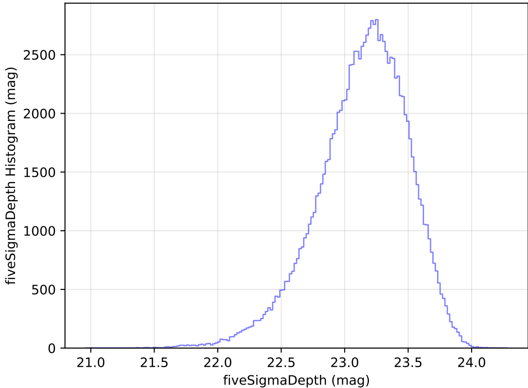
too_elab_heavy_r64_d3_gz_v3.4_10yrs All sky u band: fiveSigmaDepth Histogram
