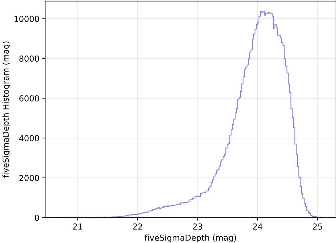
too_elab_heavy_r64_d3_gz_v3.4_10yrs All sky r band: fiveSigmaDepth Histogram
