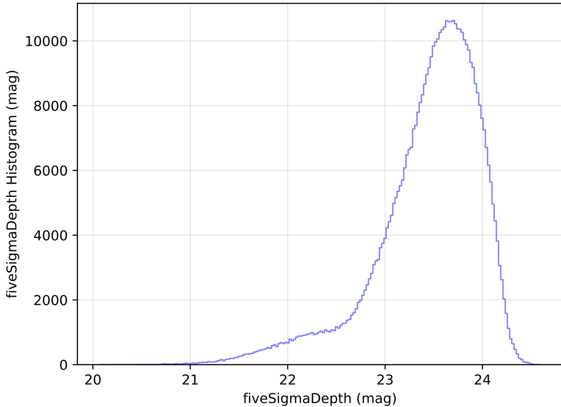
too_elab_heavy_r64_d3_gz_v3.4_10yrs All sky i band: fiveSigmaDepth Histogram
