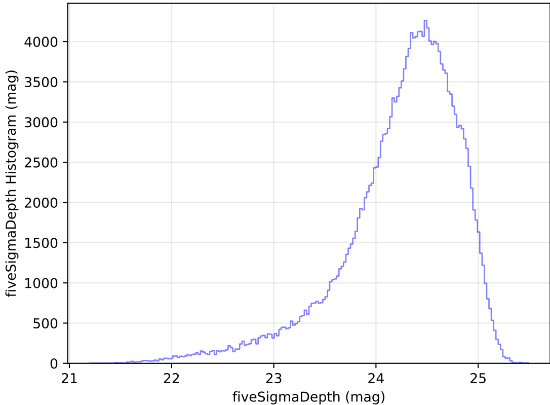
too_elab_heavy_r64_d3_gz_v3.4_10yrs All sky g band: fiveSigmaDepth Histogram
