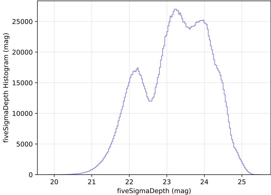
too_elab_heavy_r64_d3_gz_v3.4_10yrs All sky all bands: fiveSigmaDepth Histogram
