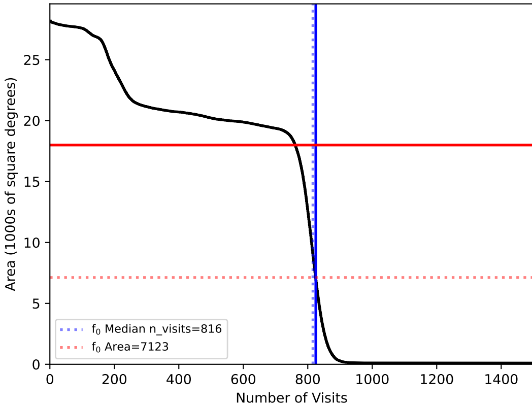
too_elab_heavy_r64_d3_gz_v3.4_10yrs All sky: f0
