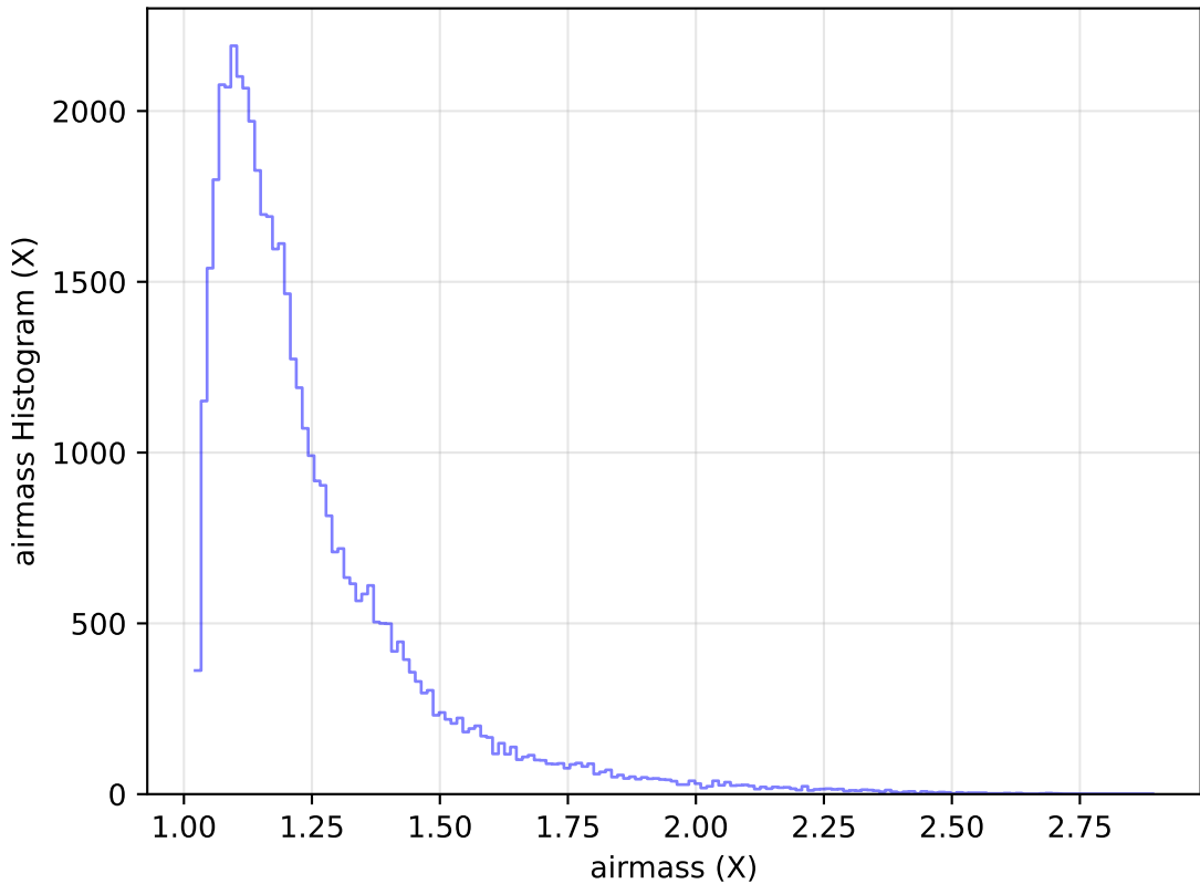
too_elab_heavy_r64_d3_gz_v3.4_10yrs Yr 1 y band: airmass Histogram
