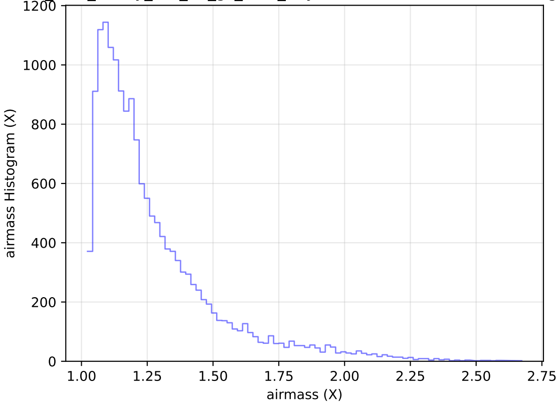
too_elab_heavy_r64_d3_gz_v3.4_10yrs Yr 1 u band: airmass Histogram
