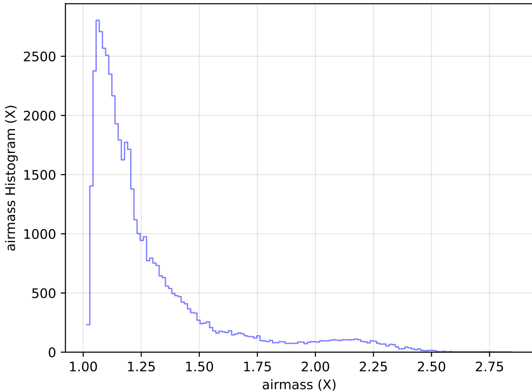
too_elab_heavy_r64_d3_gz_v3.4_10yrs Yr 1 r band: airmass Histogram
