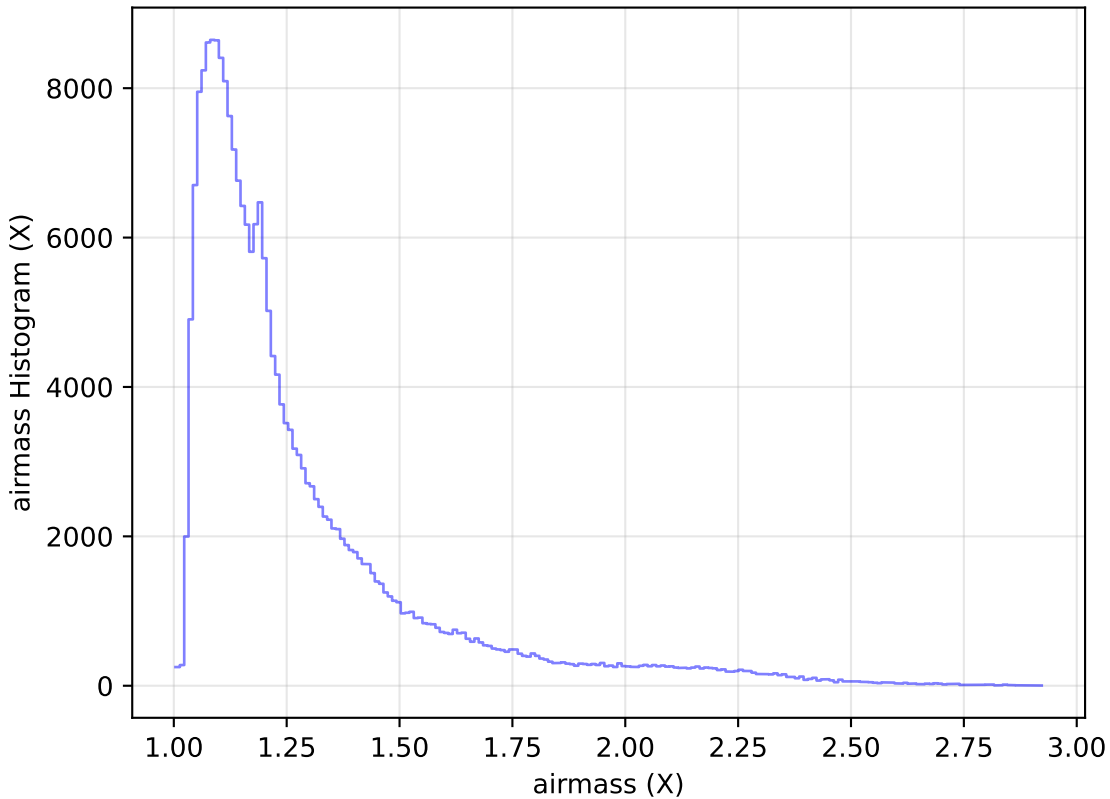
too_elab_heavy_r64_d3_gz_v3.4_10yrs Yr 1 all bands: airmass Histogram
