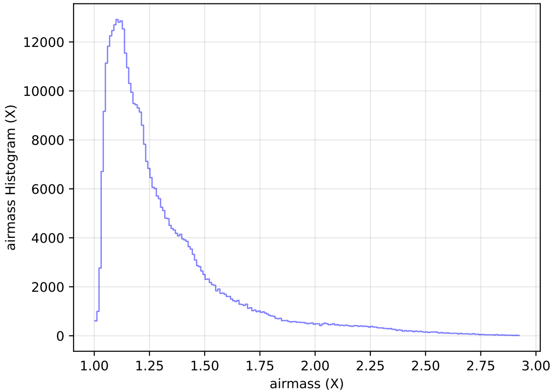
too_elab_heavy_r64_d3_gz_v3.4_10yrs WFD z band: airmass Histogram
