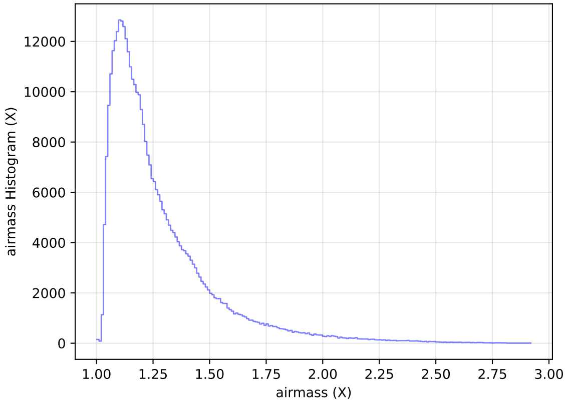
too_elab_heavy_r64_d3_gz_v3.4_10yrs WFD y band: airmass Histogram
