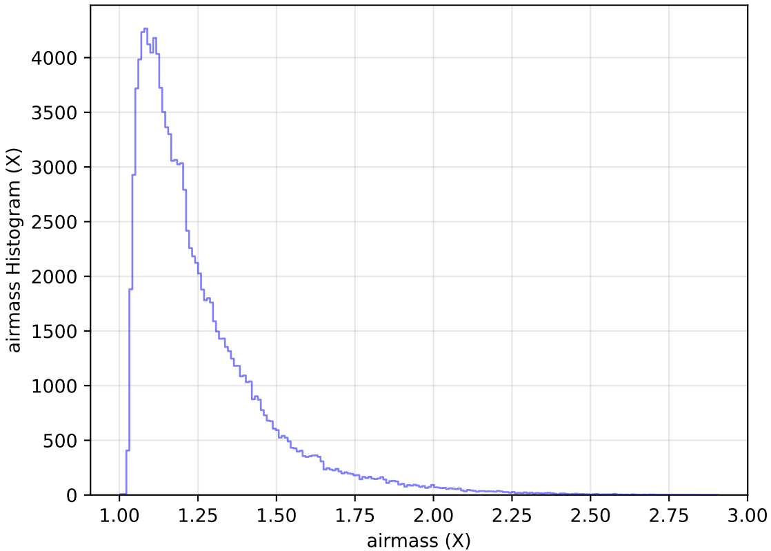
too_elab_heavy_r64_d3_gz_v3.4_10yrs WFD u band: airmass Histogram
