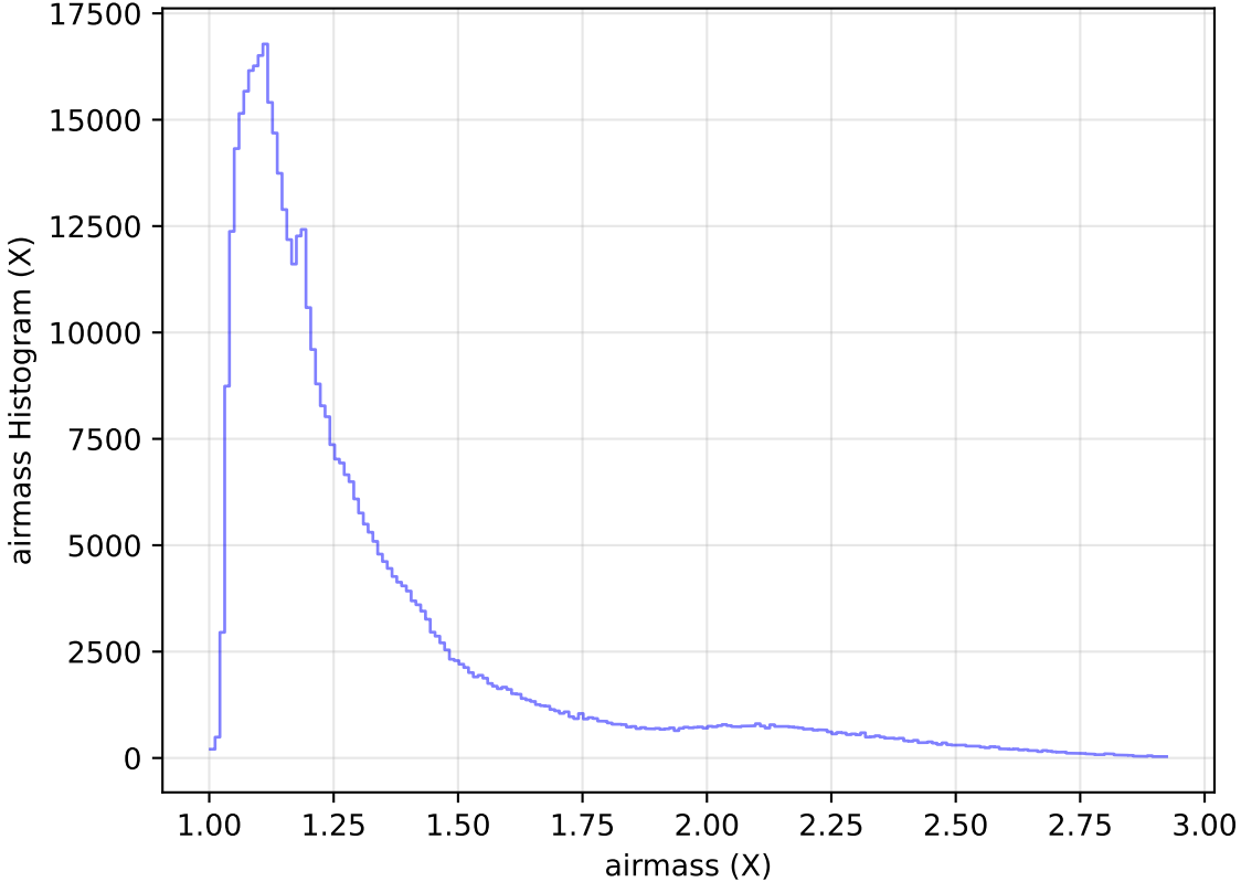
too_elab_heavy_r64_d3_gz_v3.4_10yrs WFD i band: airmass Histogram
