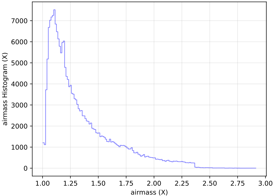
too_elab_heavy_r64_d3_gz_v3.4_10yrs WFD g band: airmass Histogram
