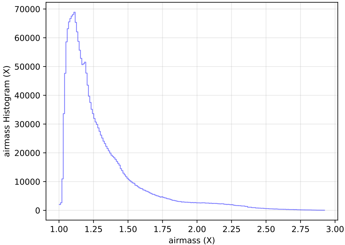
too_elab_heavy_r64_d3_gz_v3.4_10yrs WFD all bands: airmass Histogram
