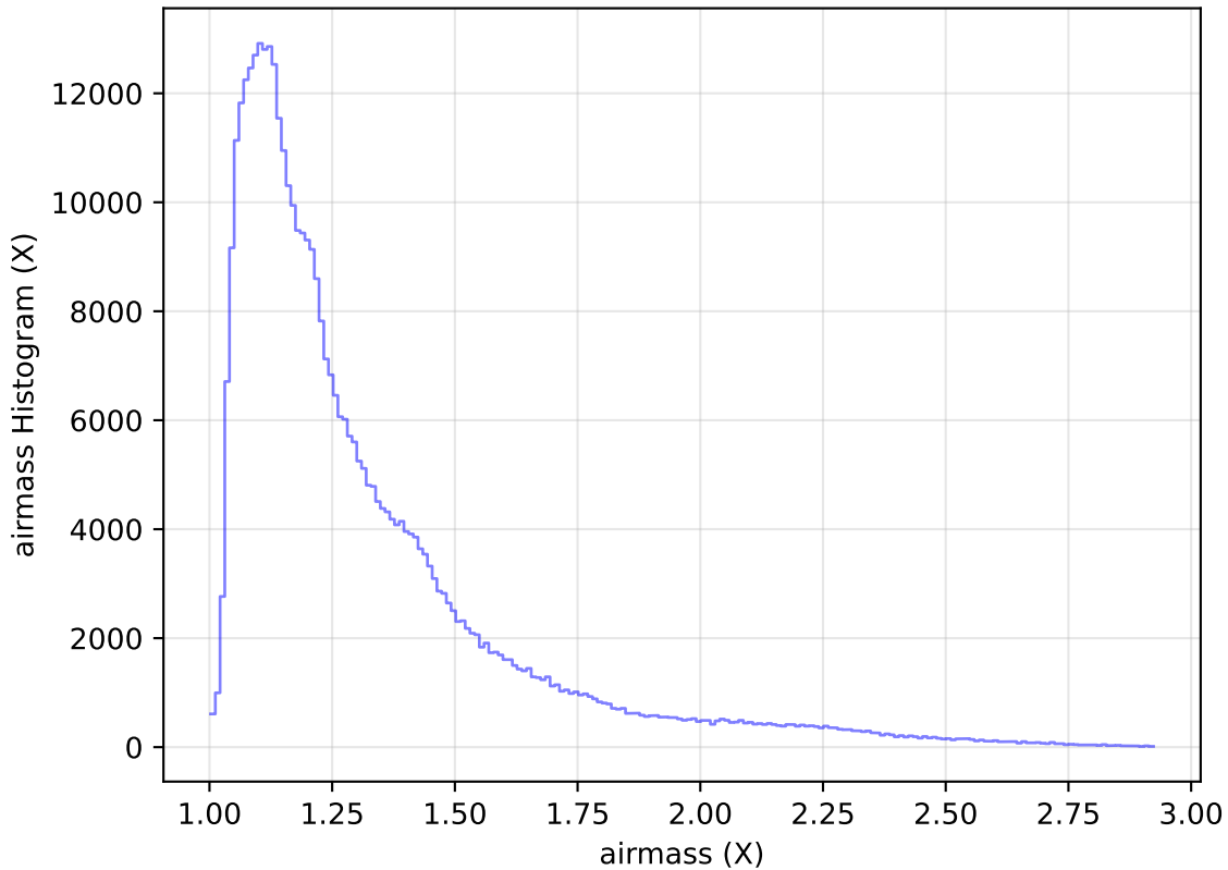
too_elab_heavy_r64_d3_gz_v3.4_10yrs All sky z band: airmass Histogram
