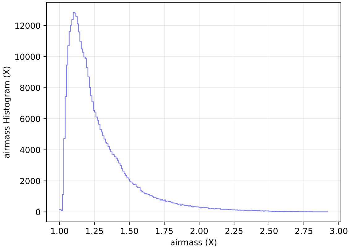
too_elab_heavy_r64_d3_gz_v3.4_10yrs All sky y band: airmass Histogram
