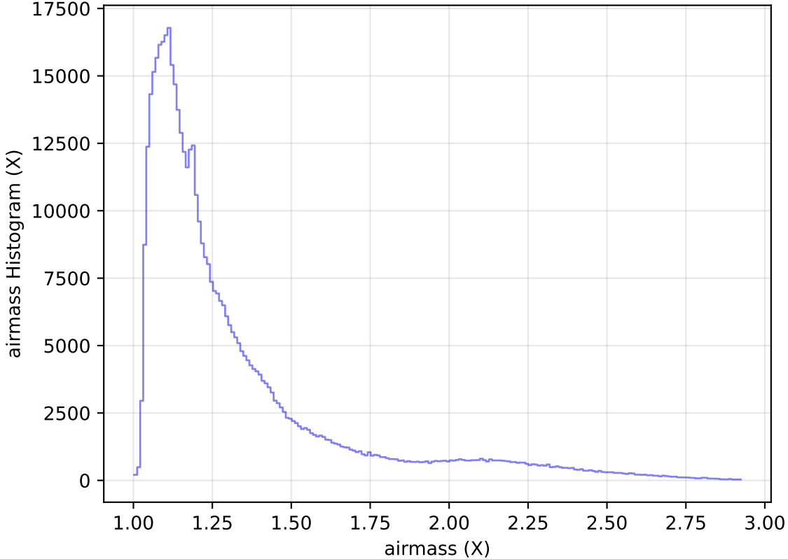
too_elab_heavy_r64_d3_gz_v3.4_10yrs All sky i band: airmass Histogram
