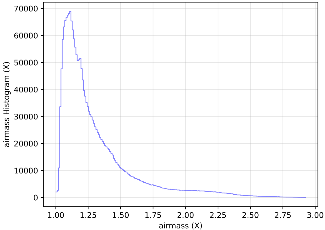
too_elab_heavy_r64_d3_gz_v3.4_10yrs All sky all bands: airmass Histogram
