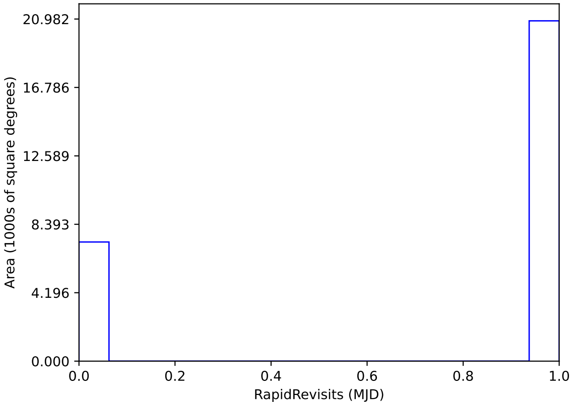
too_elab_heavy_r64_d3_gz_v3.4_10yrs All sky: RapidRevisits
