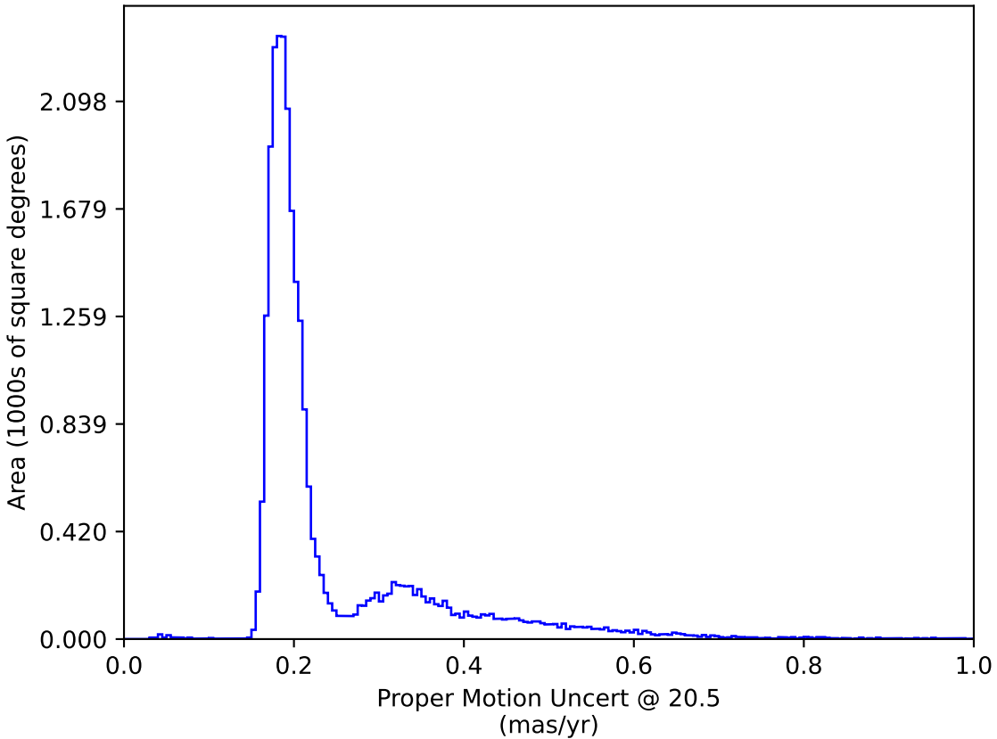
too_elab_heavy_r64_d3_gz_v3.4_10yrs All sky: Proper Motion Uncert @ 20.5
