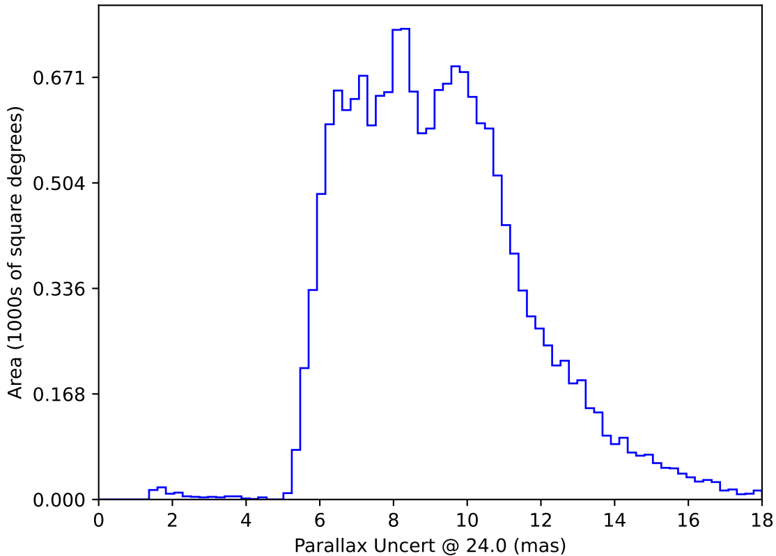
too_elab_heavy_r64_d3_gz_v3.4_10yrs WFD: Parallax Uncert @ 24.0
