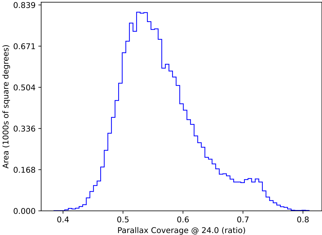
too_elab_heavy_r64_d3_gz_v3.4_10yrs WFD: Parallax Coverage @ 24.0
